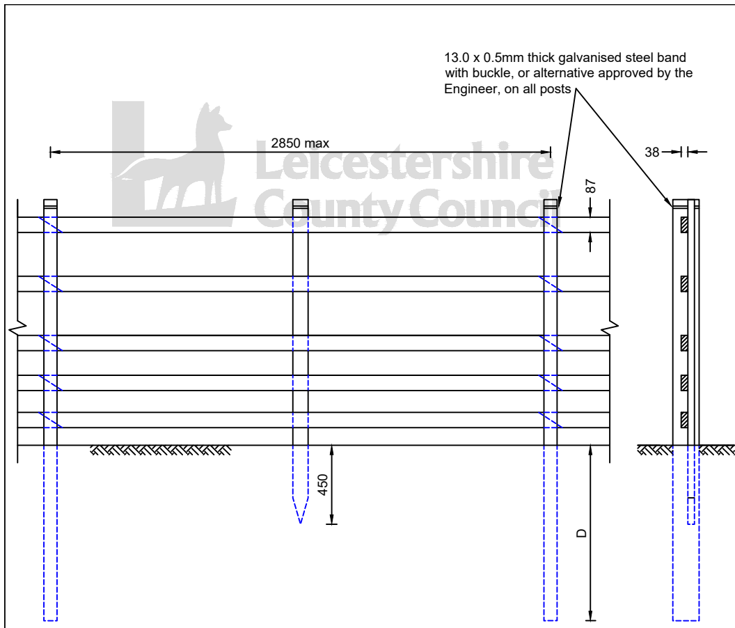
TYPICAL CONSTRUCTION DETAILS - MORTICED POST AND FIVE RAIL FENCING
