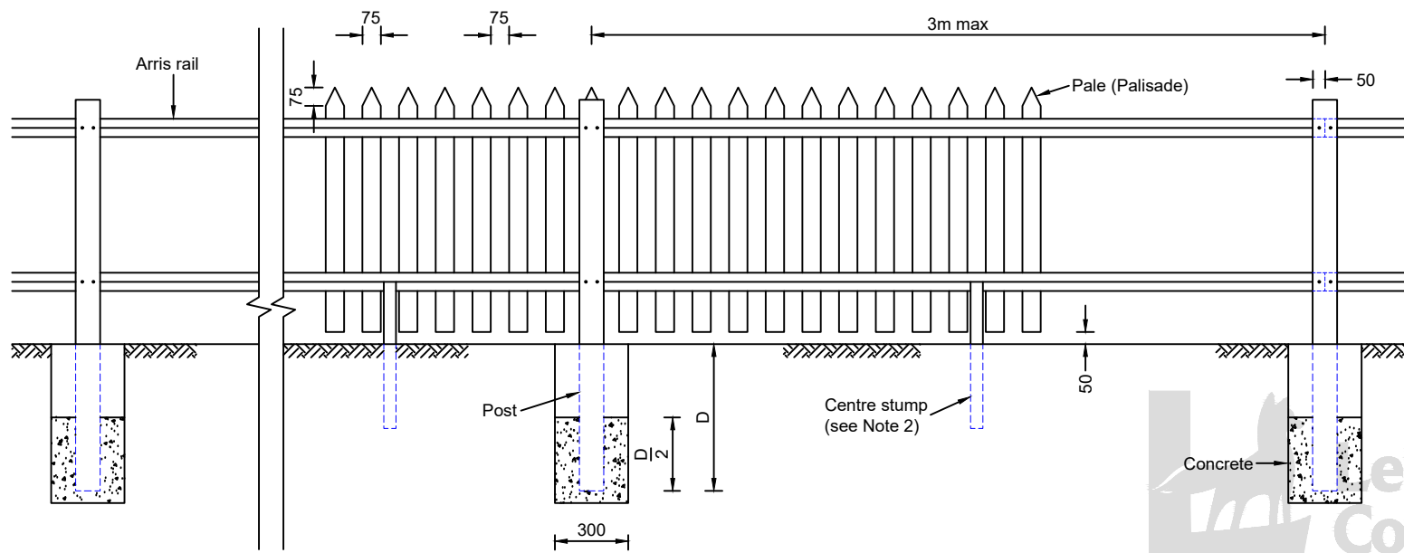
TYPICAL CONSTRUCTION DETAILS (TYPE ILLUSTRATED REF WPC 105 - CONCRETE POSTS)
