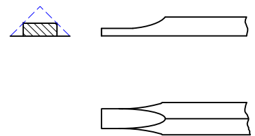
SHAPING OF ARRIS RAILS FOR MORTICE
