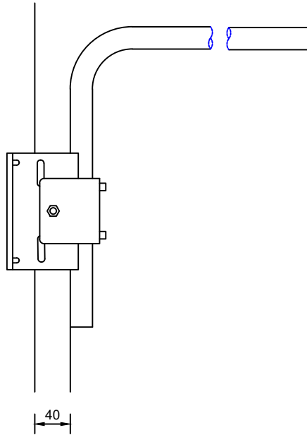
WALL BRACKET
