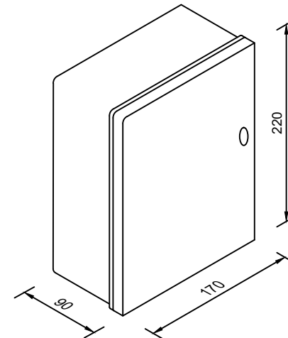
CUT-OUT BOX
