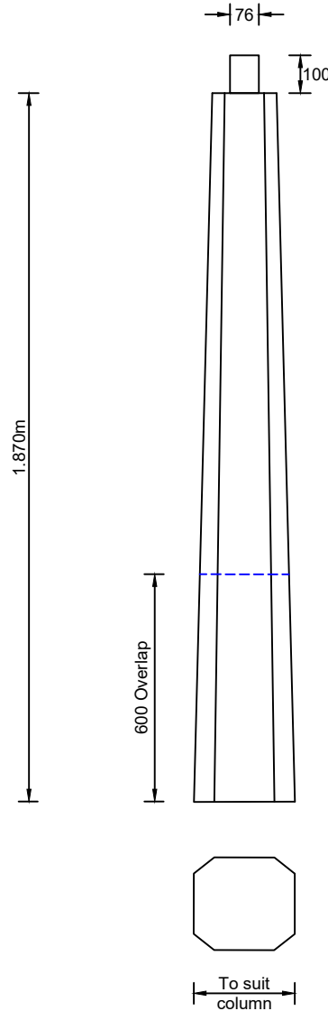
TYPICAL SLEEVE BRACKETS FOR 5/6m COLUMNS
