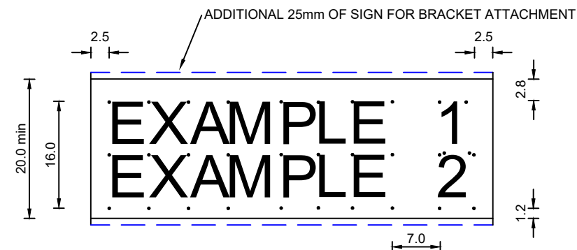
SIGN ARM WITH TWO LINES OF LEGEND
