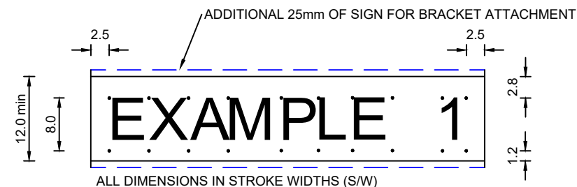
SIGN ARM WITH SINGLE LINE OF LEGEND
