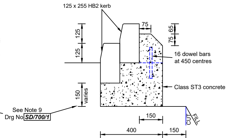
DOUBLE KERB - K19
