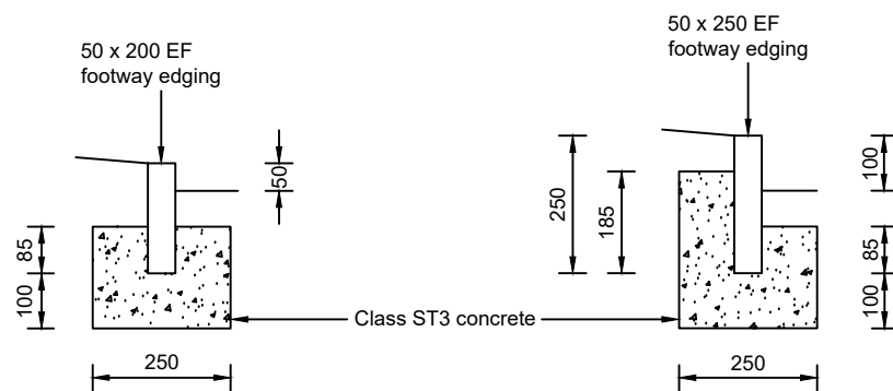
FOOTWAY EDGING EF 200
